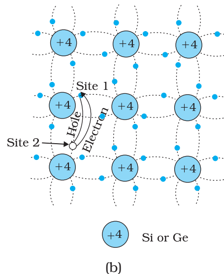
FIGURE 14.5 (a) Schematic model of generation of hole at site 1 and conduction electron due to thermal energy at moderate temperatures. (b) Simplified representation of possible thermal motion of a hole. The electron from the lower left hand covalent bond (site 2) goes to the earlier hole site 1, leaving a hole at its site indicating an apparent movement of the hole from site 1 to site 2.
