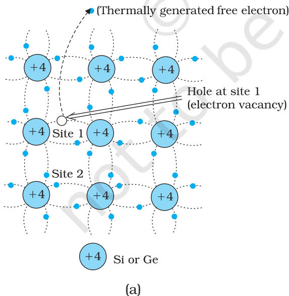
FIGURE 14.5 (a) Schematic model of generation of hole at site 1 and conduction electron due to thermal energy at moderate temperatures. (b) Simplified representation of possible thermal motion of a hole. The electron from the lower left hand covalent bond (site 2) goes to the earlier hole site 1, leaving a hole at its site indicating an apparent movement of the hole from site 1 to site 2.
