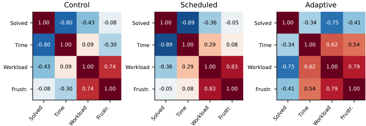
Figure 6: Spearman correlations between participant-condition averages. Cells show correlation coefficients from -1 to 1 ; no significance threshold is applied. Frustration is one component of overall workload.
