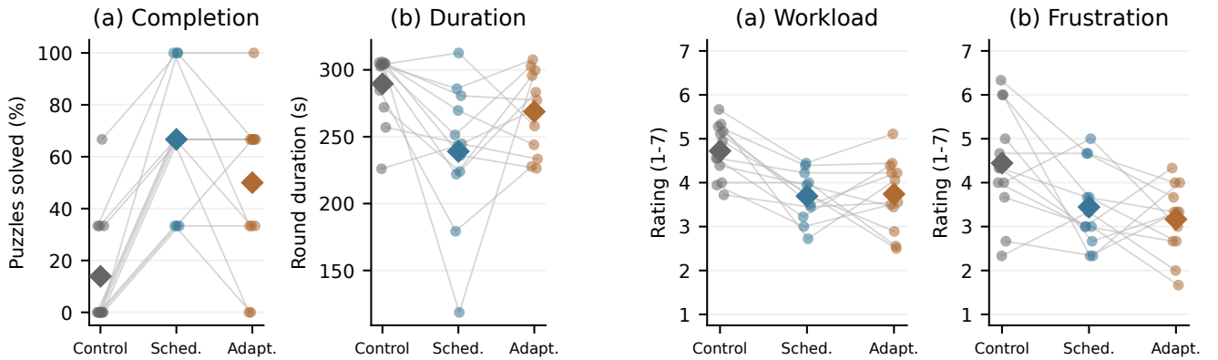
Figure 4: Puzzle completion and mean round duration. Gray lines connect the same participant across conditions; colored diamonds show condition means.
