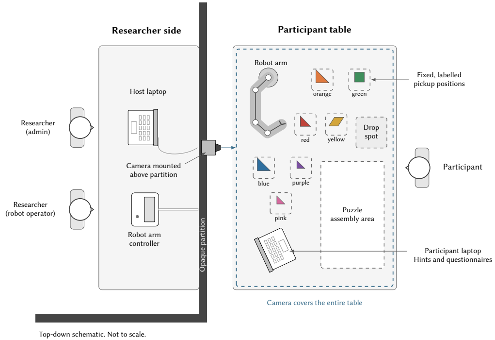
Figure 3: Top-down view of the Wizard-of-Oz setup. An opaque partition separates the researchers from the participant; a camera mounted on the partition observes the participant table. The table contains fixed piece pickup positions, the robot drop spot, the assembly area, and the participant laptop. Schematic not to scale.
