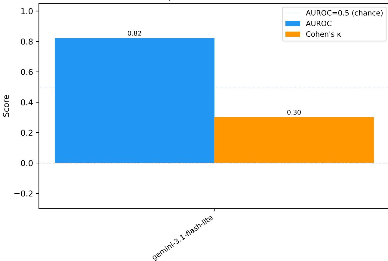
Model Comparison — AUROC & Cohen's \kappa
