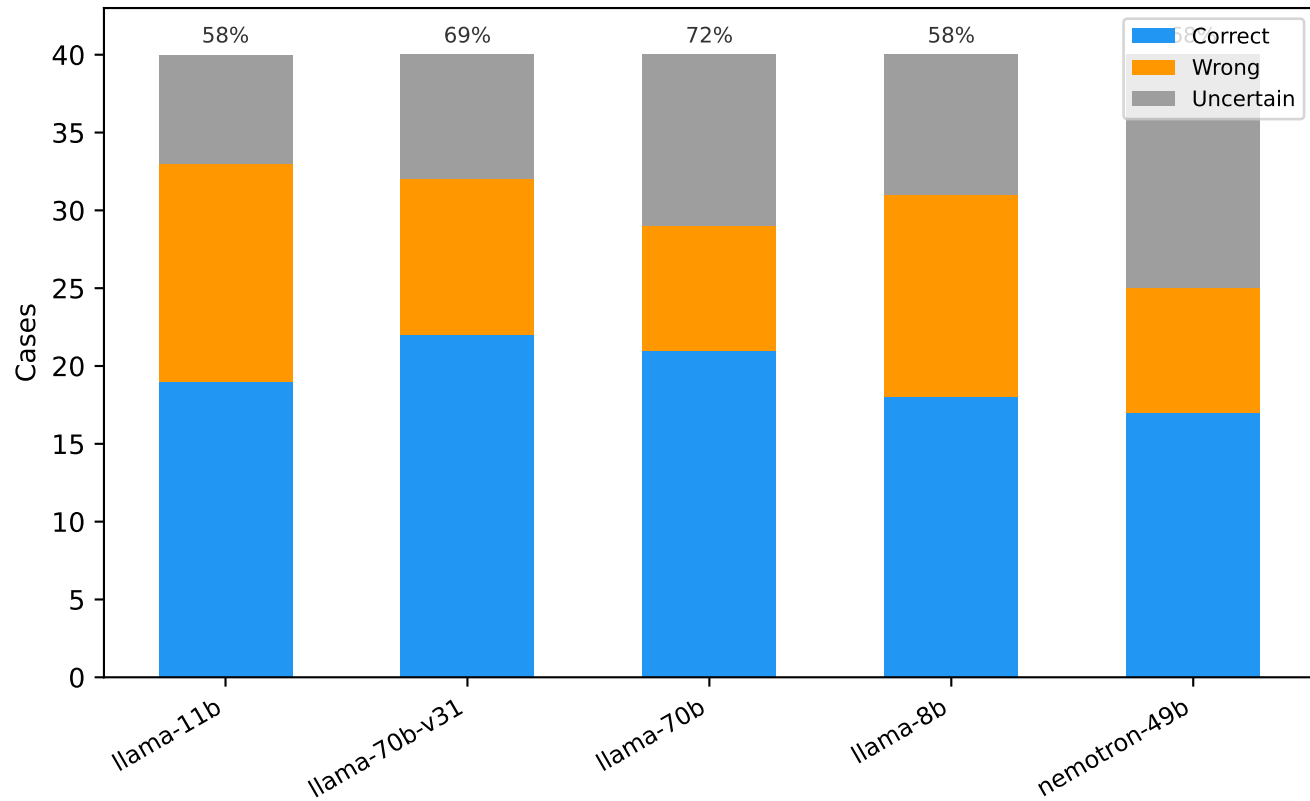
Prediction Outcomes (accuracy excl. uncertain shown above)
