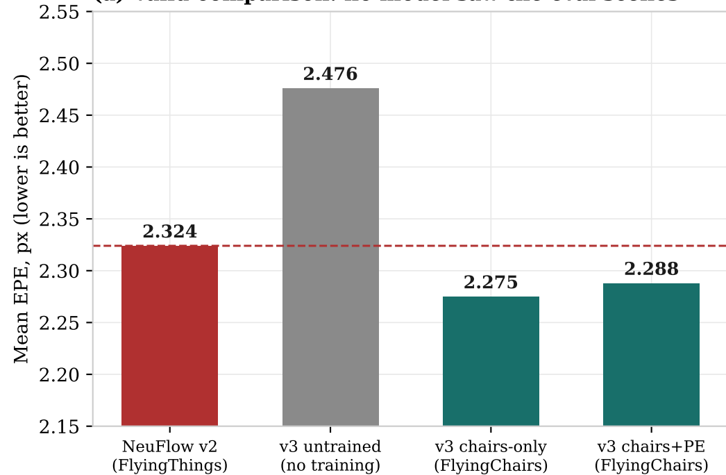
(a) Valid comparison: no model saw the eval scenes
