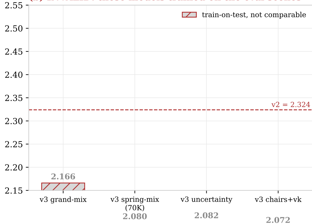
(b) INVALID: these models trained on the eval scenes
