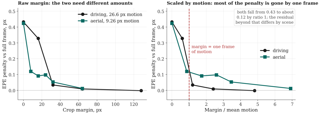
Fig. 6. Left: in raw pixels the two domains need different margins. Right: expressed as a multiple of mean inter-frame motion, both shed the bulk of the penalty by a ratio of one. Measured with the baseline network, since the effect belongs to the architecture family rather than to the decoder.
