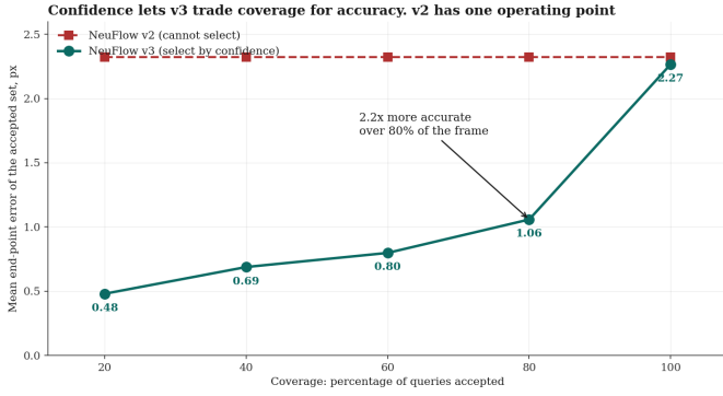
Fig. 4. Risk-coverage behaviour. The baseline has one operating point because it cannot indicate which outputs to trust; per-query confidence gives the decoder a curve.
