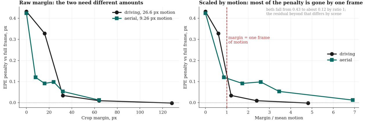
Fig. 4. Left: in raw pixels the two domains need different margins. Right: expressed as a multiple of mean inter-frame motion, both shed the bulk of the penalty by a ratio of one. Measured with the baseline network, since the effect belongs to the architecture family rather than to the decoder.
