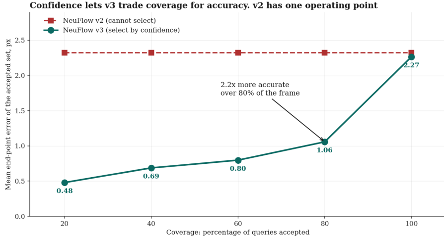
Fig. 3. Risk-coverage behaviour. The baseline has one operating point because it cannot indicate which outputs to trust; per-query confidence gives the decoder a curve.
