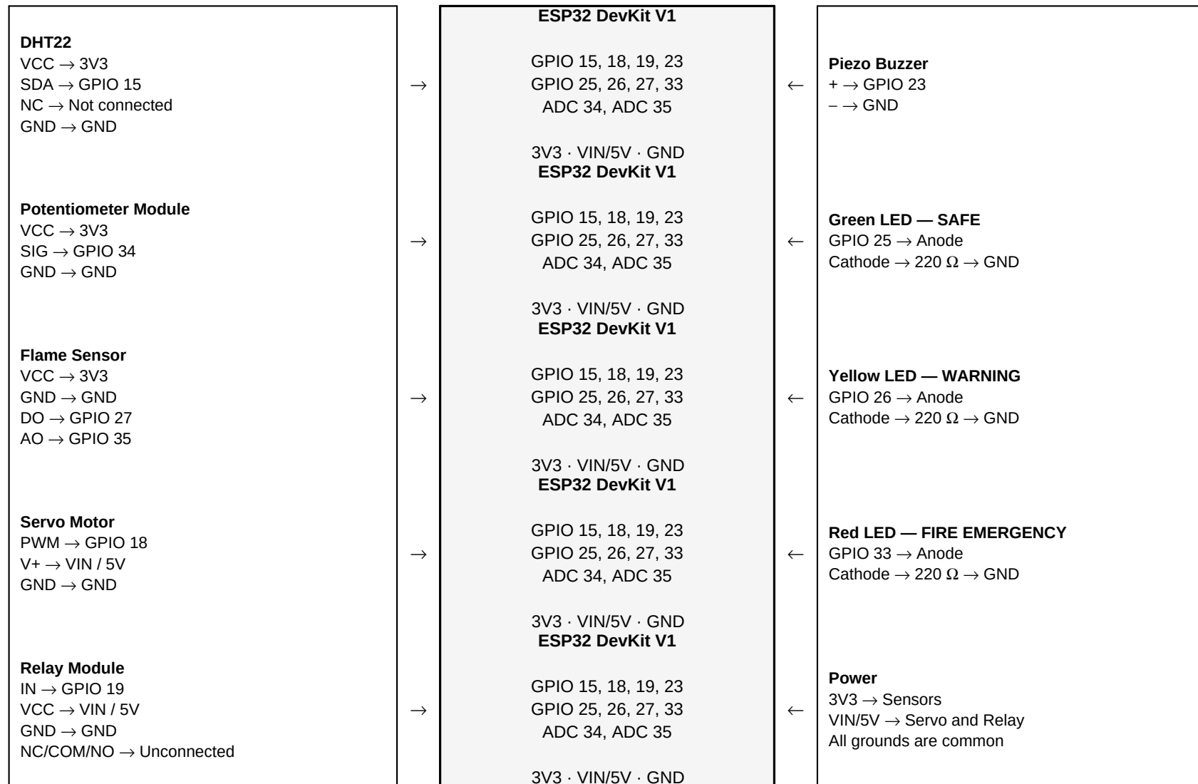
Schematic / Wiring Connection Diagram
