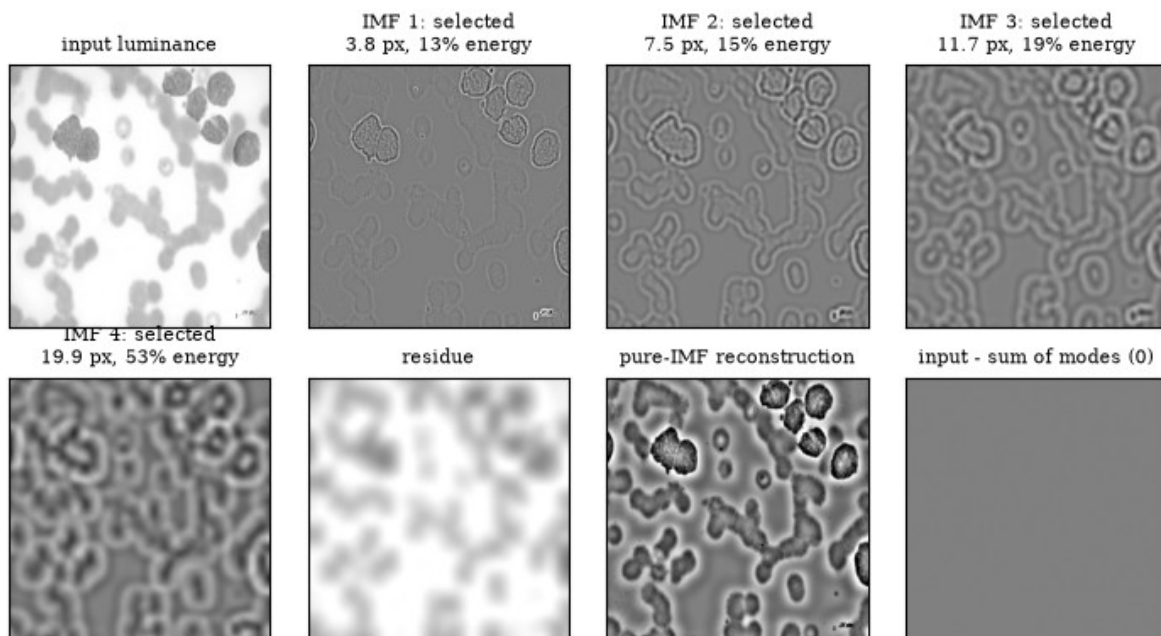
Figure 8. Stages 6 and 7, BEEMD and pure-IMF selection for the luminance of WBC-Malignant-Early-025. The four intrinsic mode functions (IMFs) are ordered from fine to coarse; the title of each gives the characteristic spatial period, the share of the detail energy and whether the selection rule keeps the mode. Also shown: the residue, the sum of the selected (pure) modes, and the difference between the input and the sum of all modes and the residue, which is zero up to rounding.
