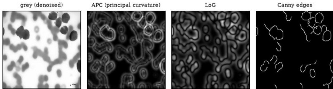
Figure 7. Stage 4, response layers of WBC-Malignant-Early-025. From left to right: denoised grey image, adaptive principal-curvature (APC) response, Laplacian-of-Gaussian (LoG) response and Canny edges.
