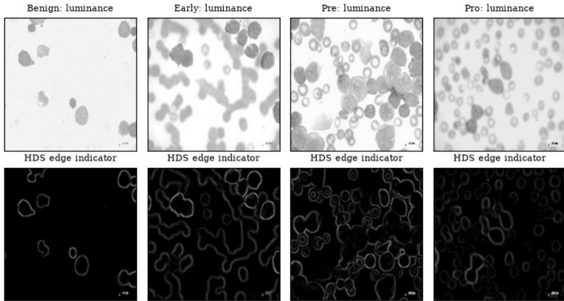
Figure 6. Stage 3, HDS edge indicator. Top: luminance of one image per class. Bottom: the edge indicator 1 - \text{mean diffusivity of the denoised image} (0 in flat regions, close to 1 across strong edges), on a fixed scale.
