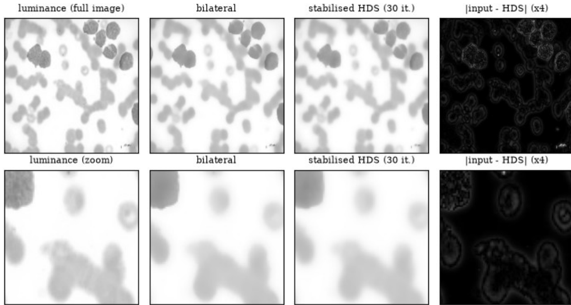
Figure 5. Stage 2, denoising of the luminance of WBC-Malignant-Early-025 (top: full image; bottom: zoom on the central region). From left to right: input, bilateral filter, stabilised HDS diffusion (30 iterations), and the absolute difference between input and HDS output (amplified four times). Diffusion smooths flat regions and leaves the cell boundaries.
