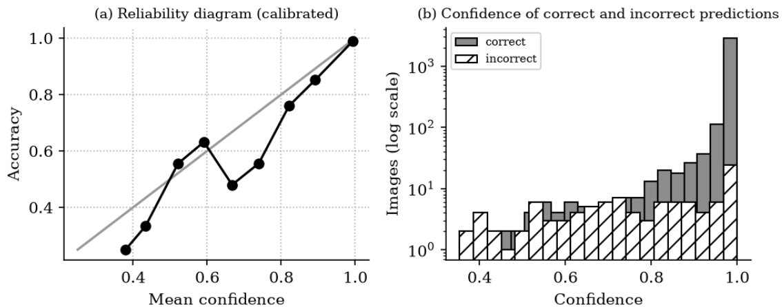
Figure 20. Calibration of the temperature-scaled probabilities on the pooled out-of-fold predictions. (a) Reliability diagram: observed accuracy against mean confidence in ten confidence bins; the diagonal is perfect calibration. (b) Histogram of the confidence of correct and incorrect predictions (log scale).
