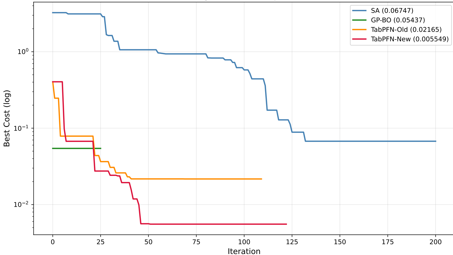
Convergence — All Optimizers
