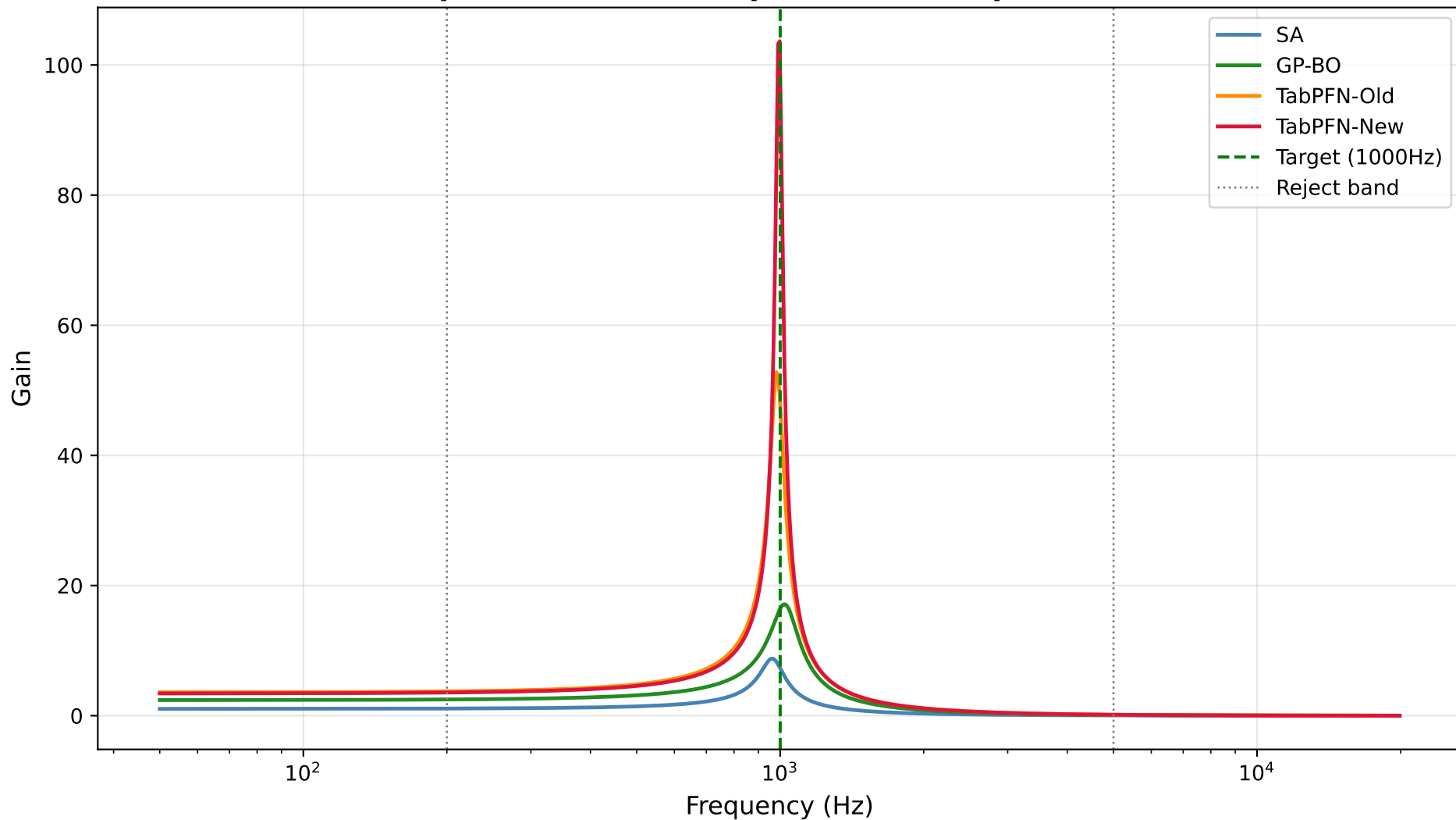
Optimized Filter Responses — All Optimizers
