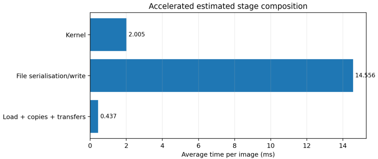
Figure 2. Average accelerated Total components derived from the 41 displayed rows. Rounding may change the final few microseconds.
