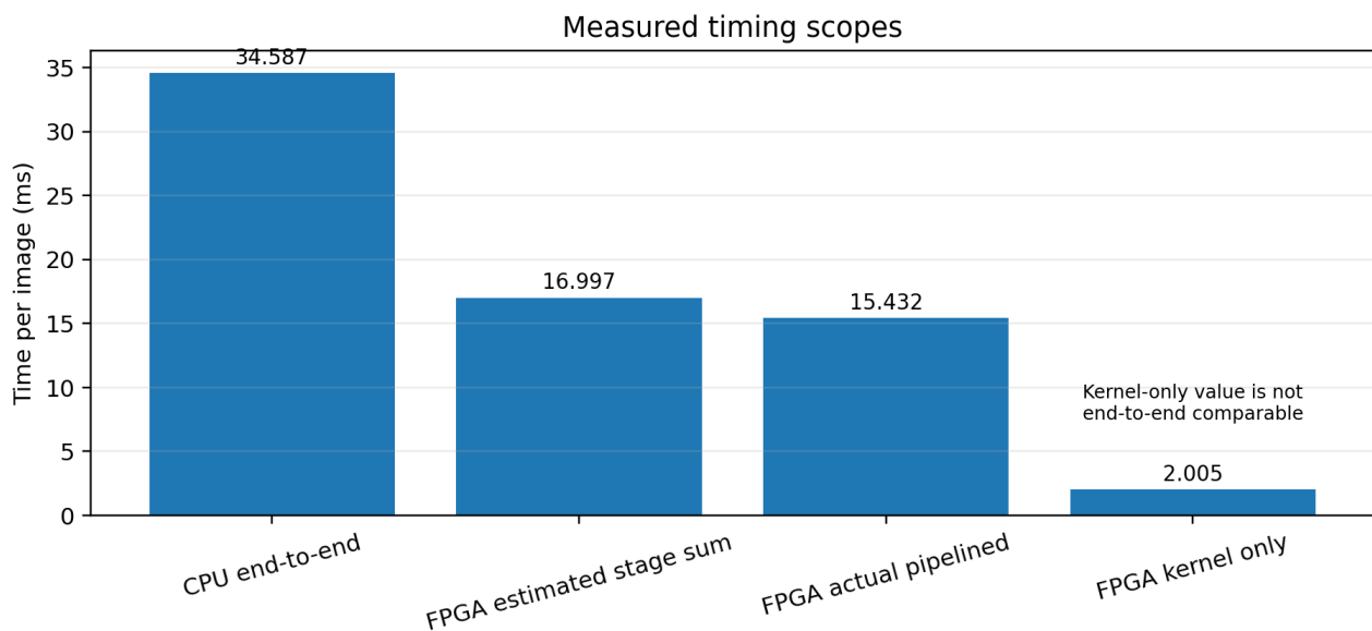
Figure 1. Timing scopes recreated from the supplied CPU and accelerated terminal results.
