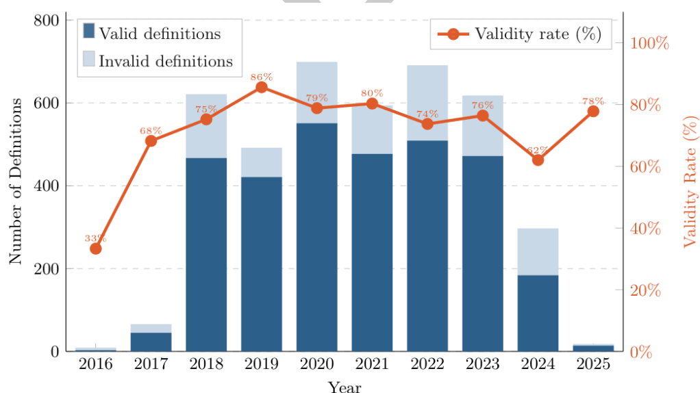
Figure 2: Validity Rates of the Pipeline
