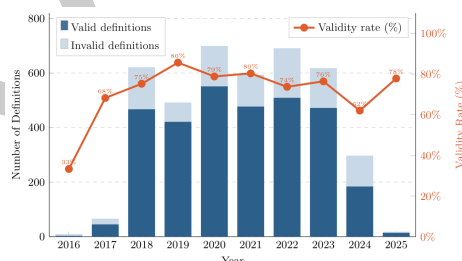
Figure 2: Extraction validity rate by year across 4,105 definitions extracted from 600 cases. Overall validity rate was found to be 76.6%.
