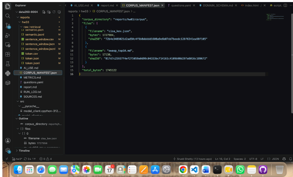
Corpus manifest
