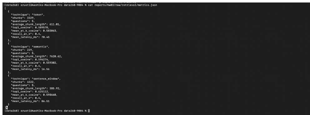
Retrieval metrics
