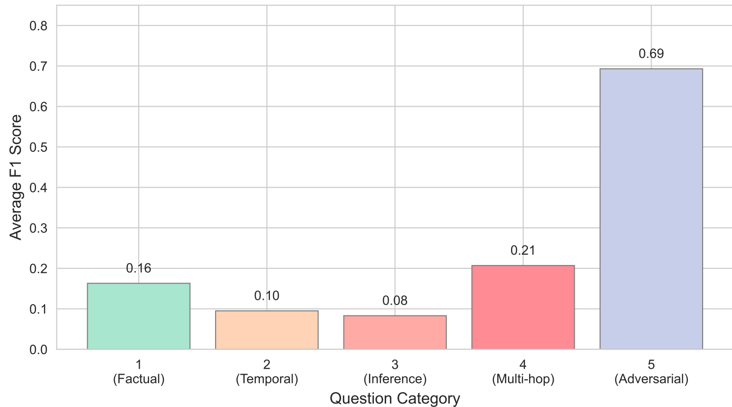
Per-Category Performance of Llama-3.1-8B (Truncated)
