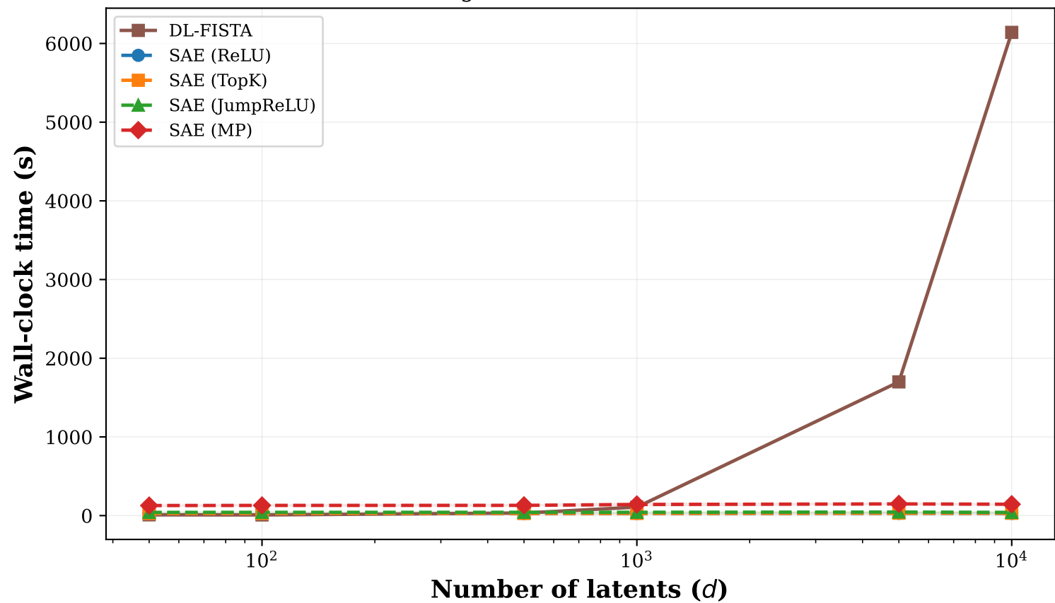
Running time vs. number of latents
