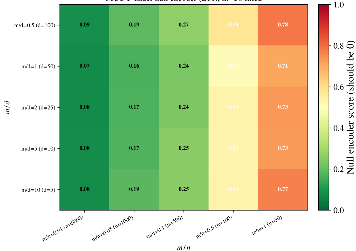
MCC-P under null encoder (E10), m=50 fixed
