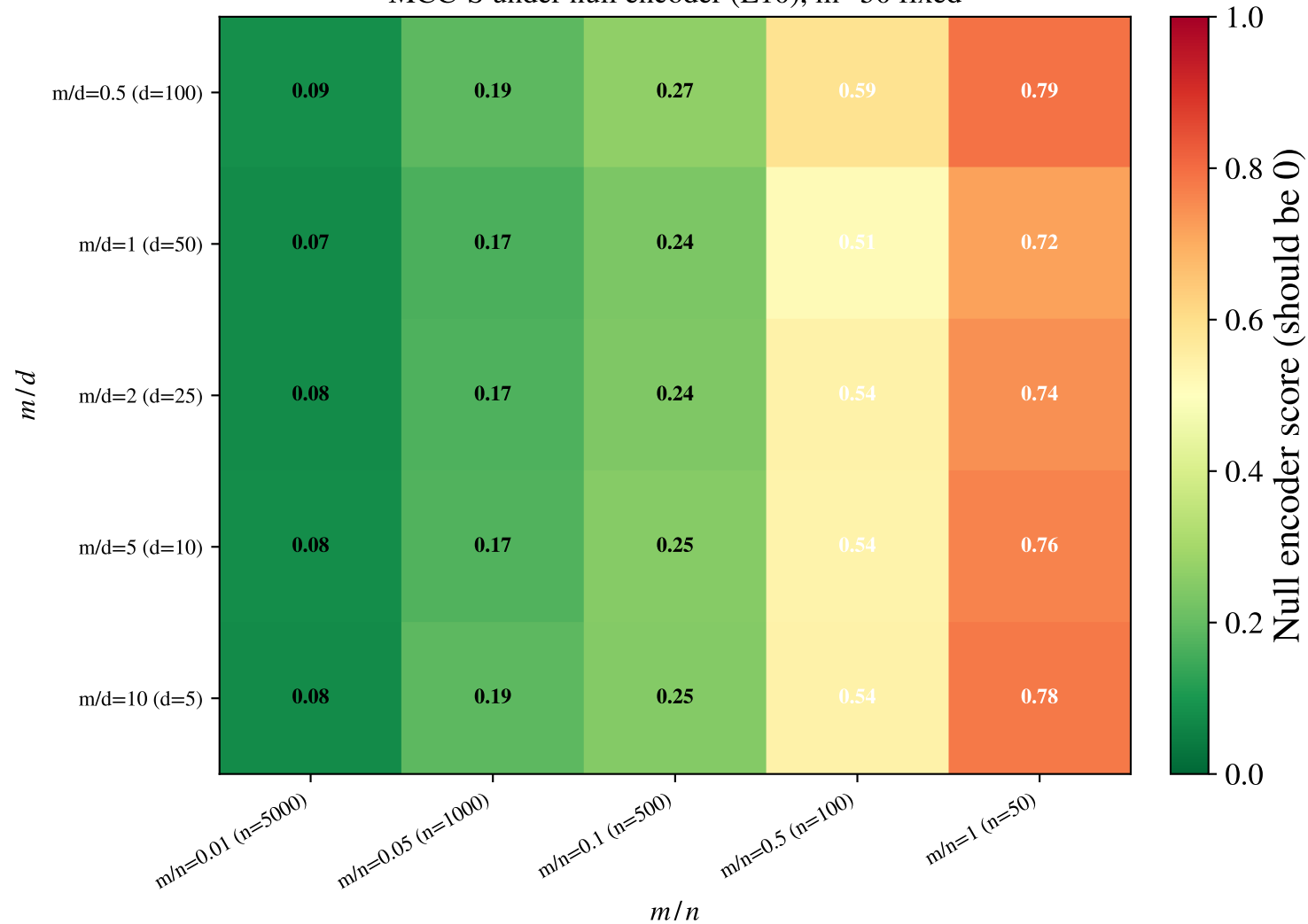
MCC-S under null encoder (E10), m=50 fixed
