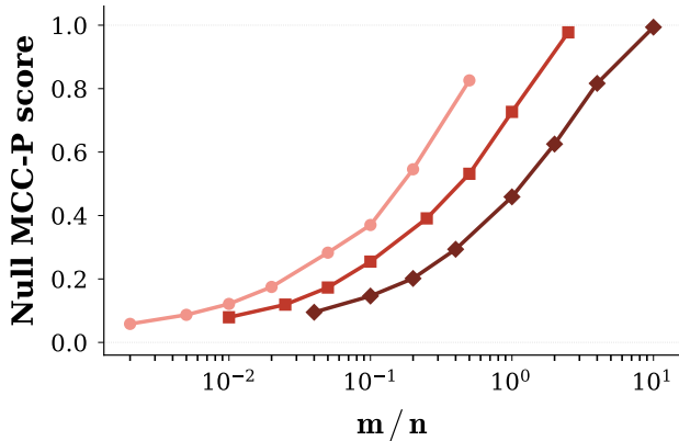
no collapse in m/n
