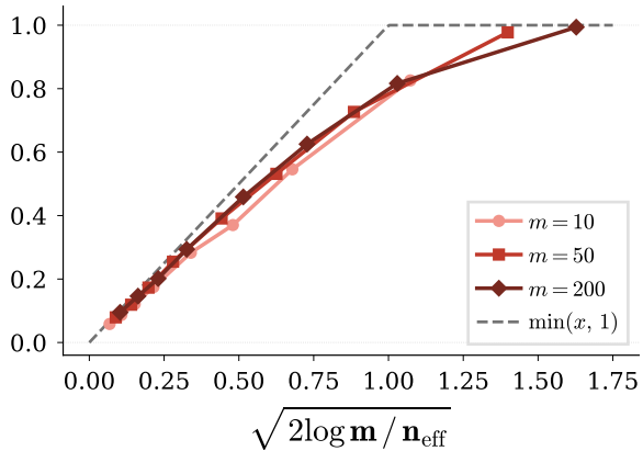
collapse in \sqrt{2\log m/n_{\text{eff}}}
