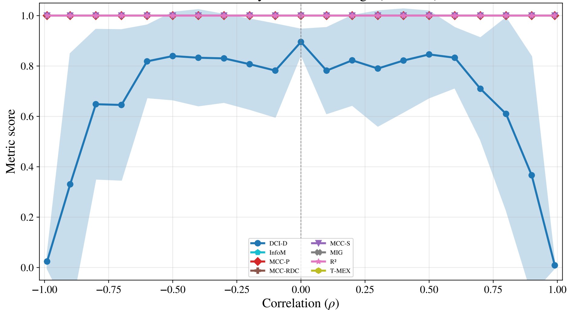
Metric sensitivity to correlation sign (D2 + E1)
