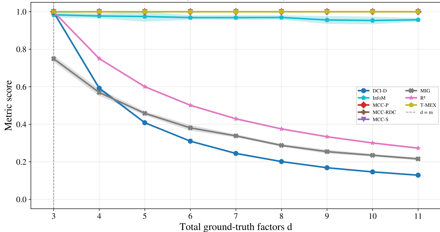
Metric inflation with extra dimensions (D1 + E4, m=3 fixed)
