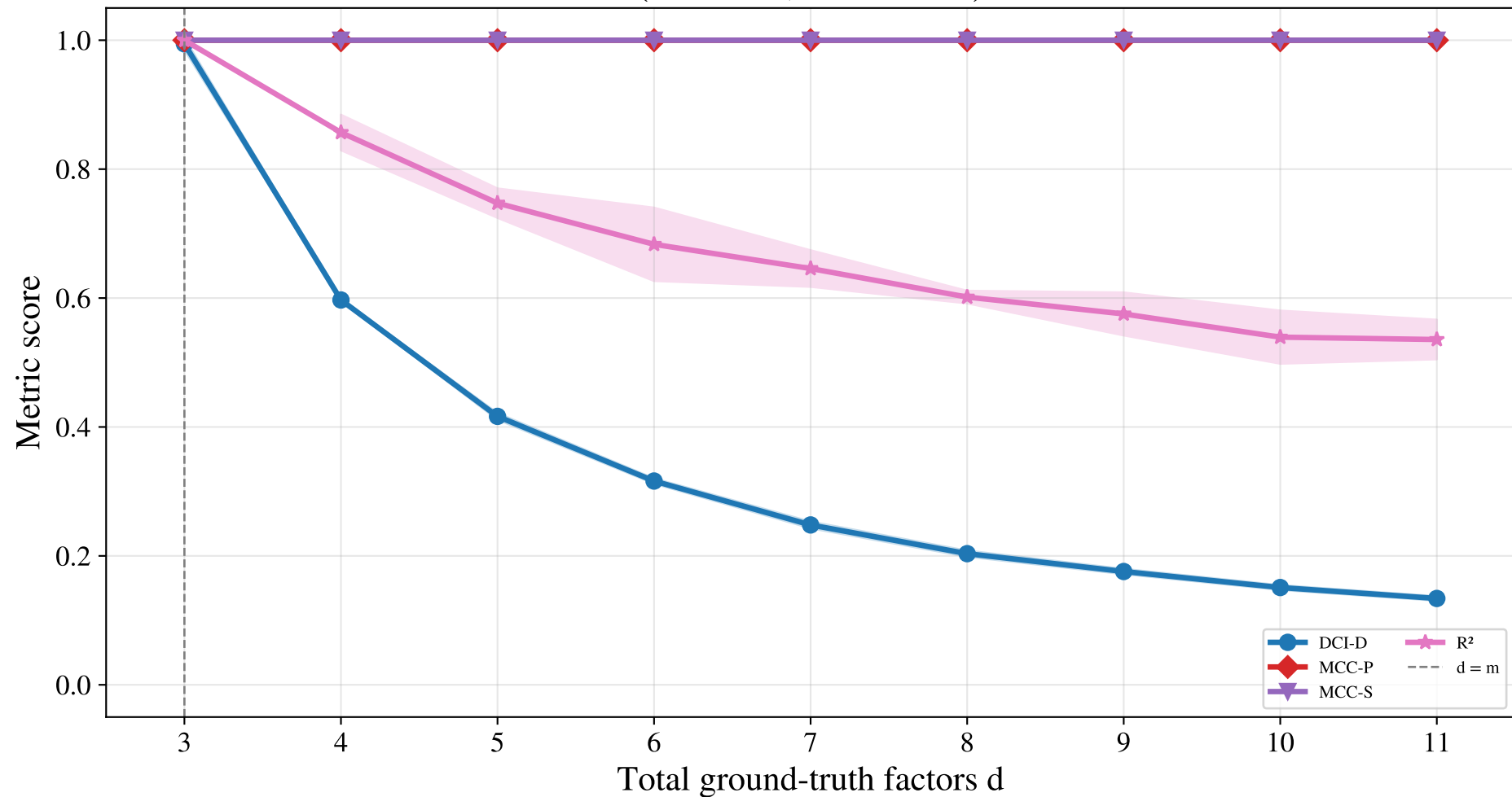
Metric inflation with extra dimensions (D2 + E4, m=3 fixed)
