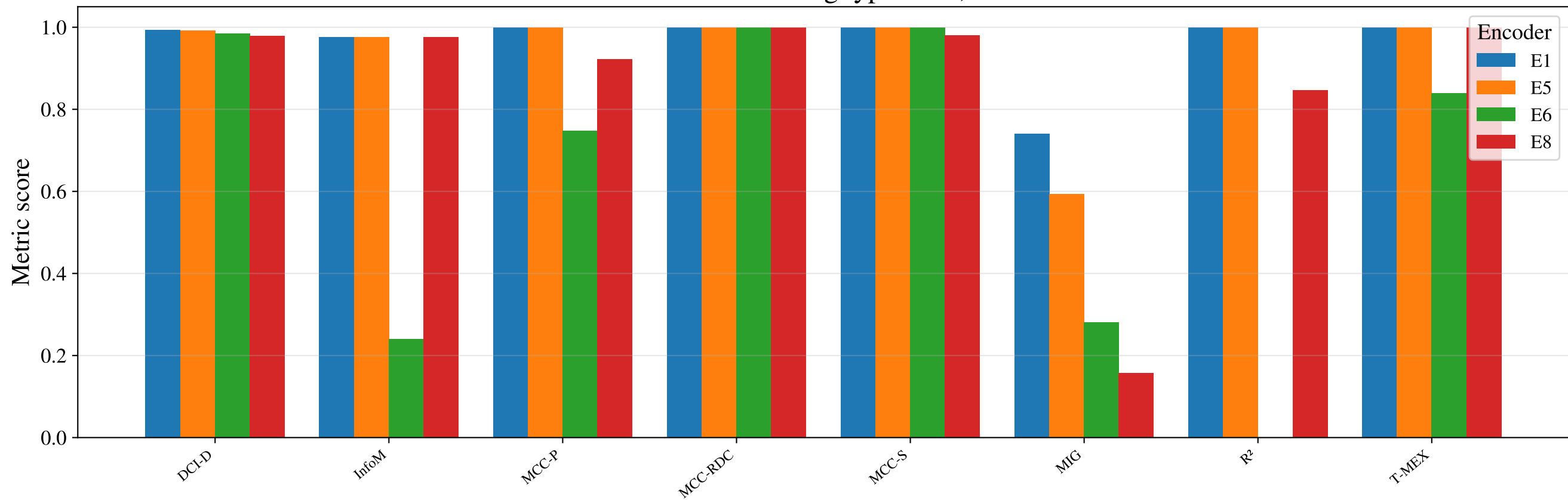
Effect of encoding type – D1, d=5
