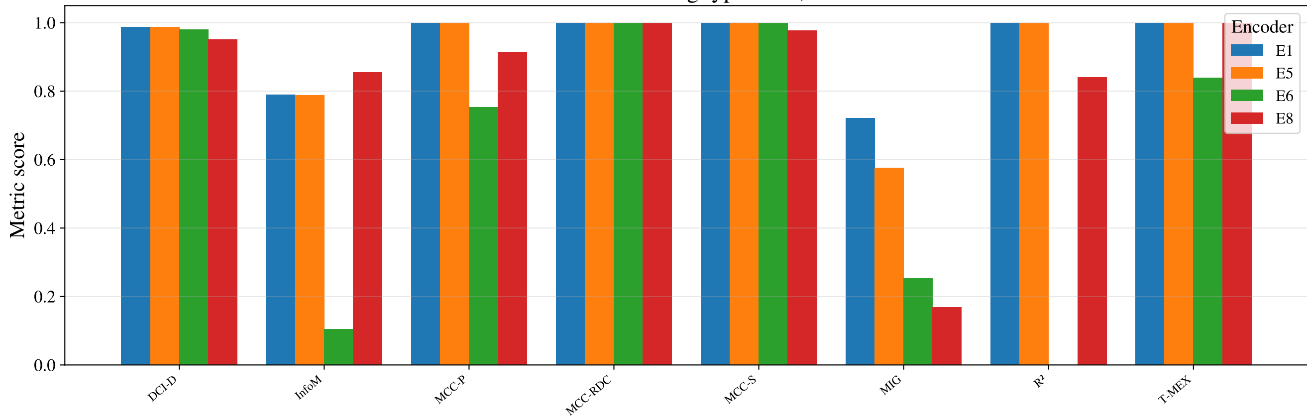
Effect of encoding type – D2, d=5
