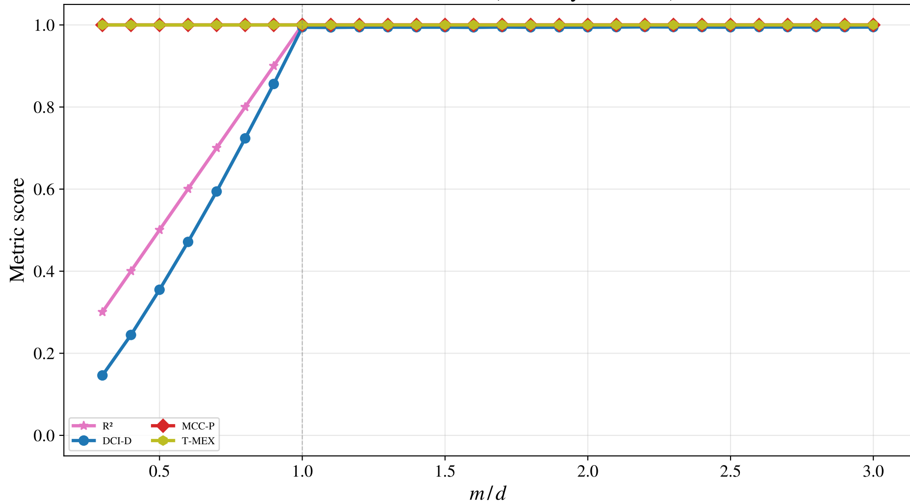
Metric score vs m/d (D1, vary m , d=10 )
