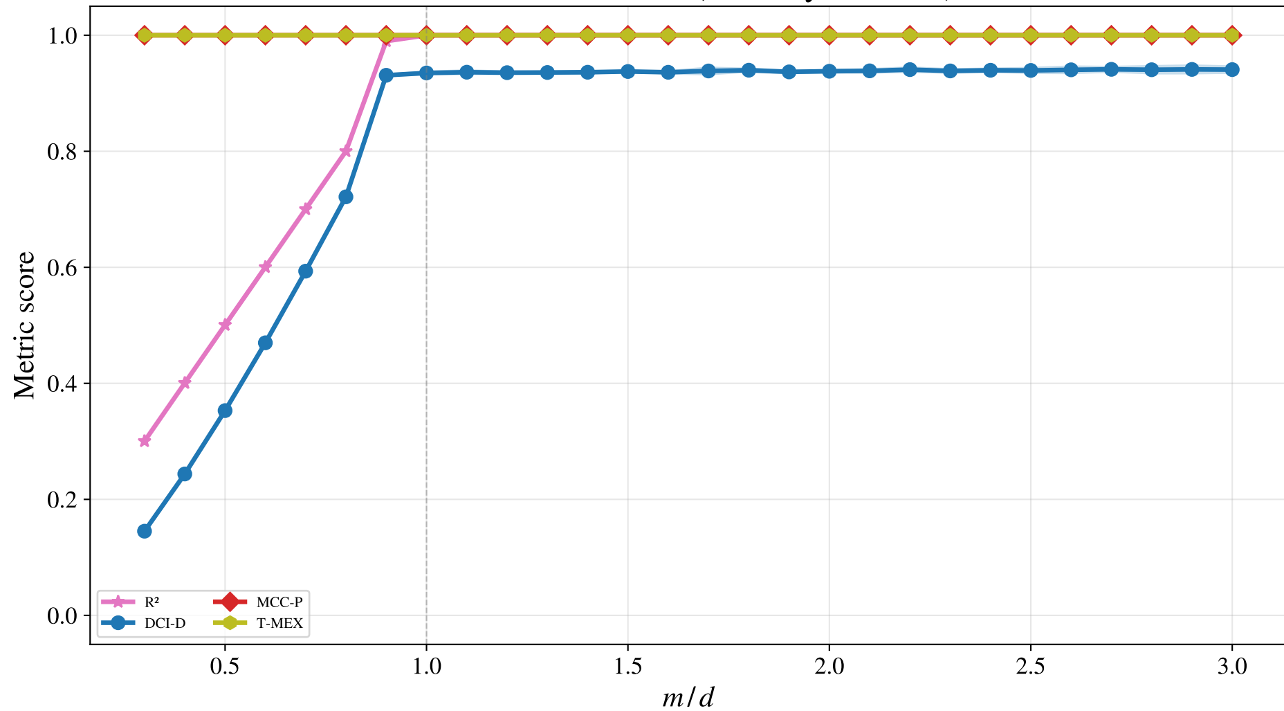
Metric score vs m/d (D3, vary m , d=10 )
