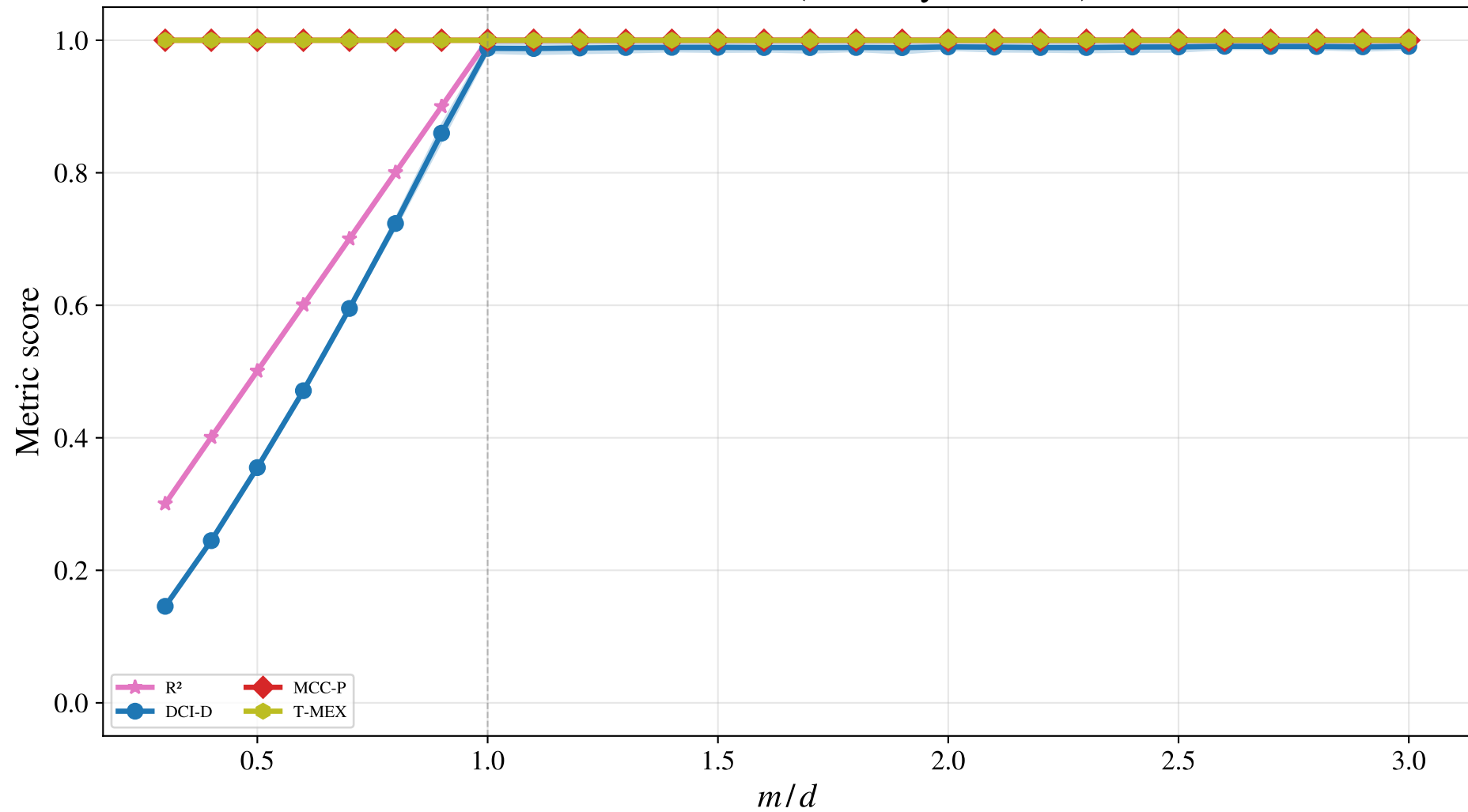
Metric score vs m/d (D4, vary m , d=10 )
