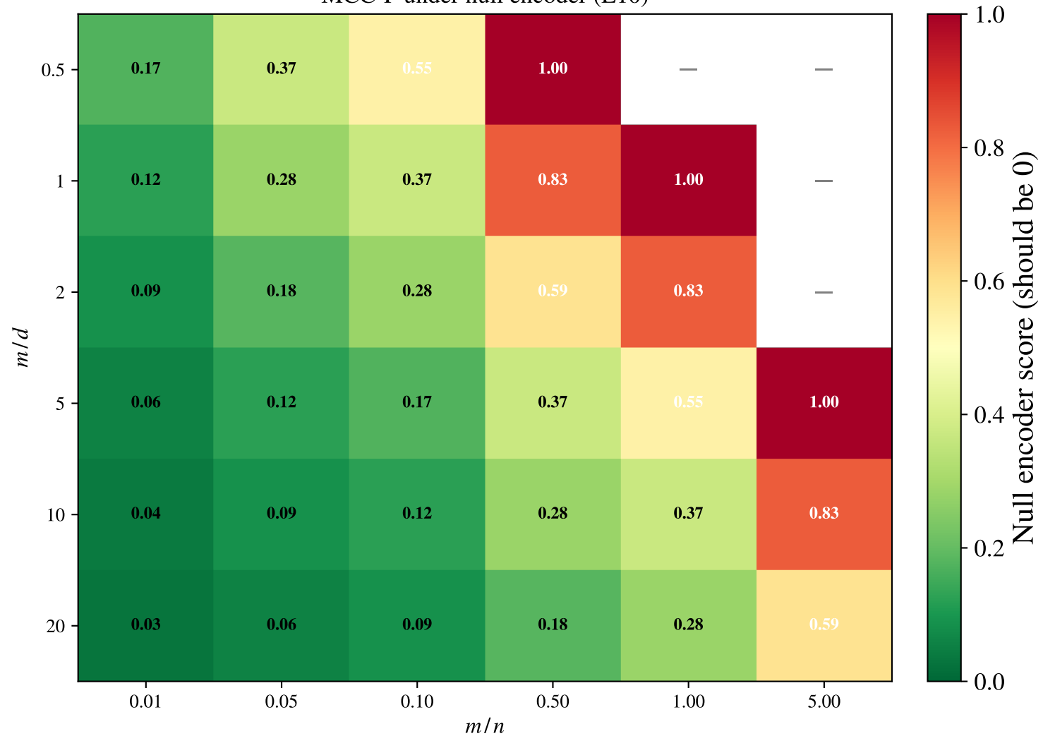
MCC-P under null encoder (E10)
