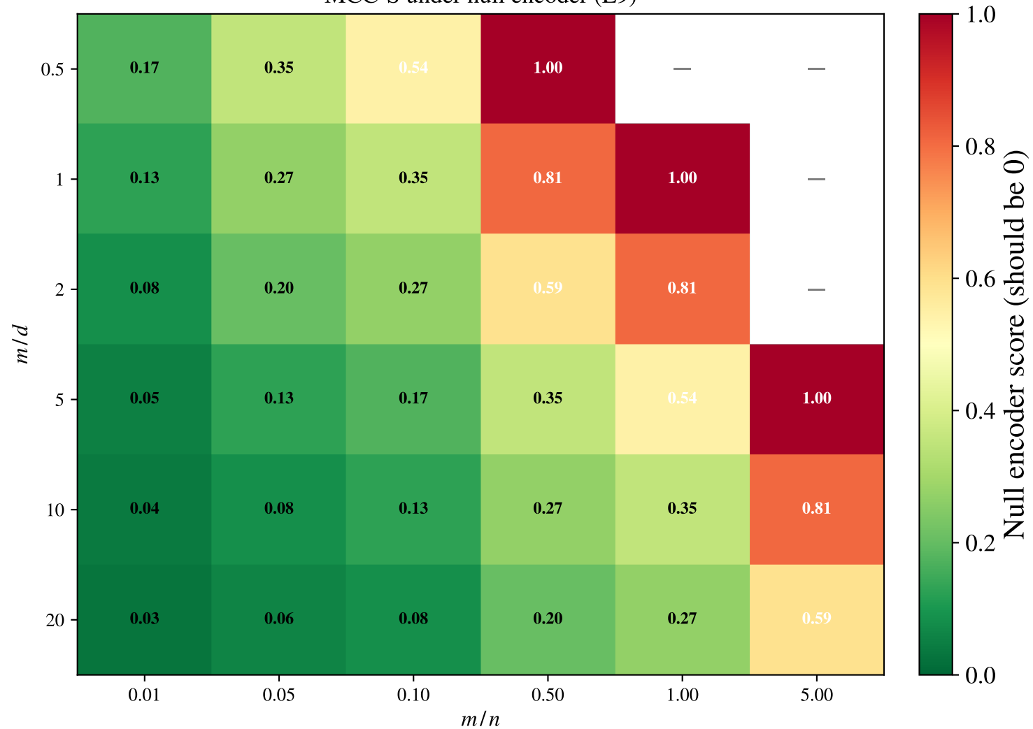
MCC-S under null encoder (E9)
