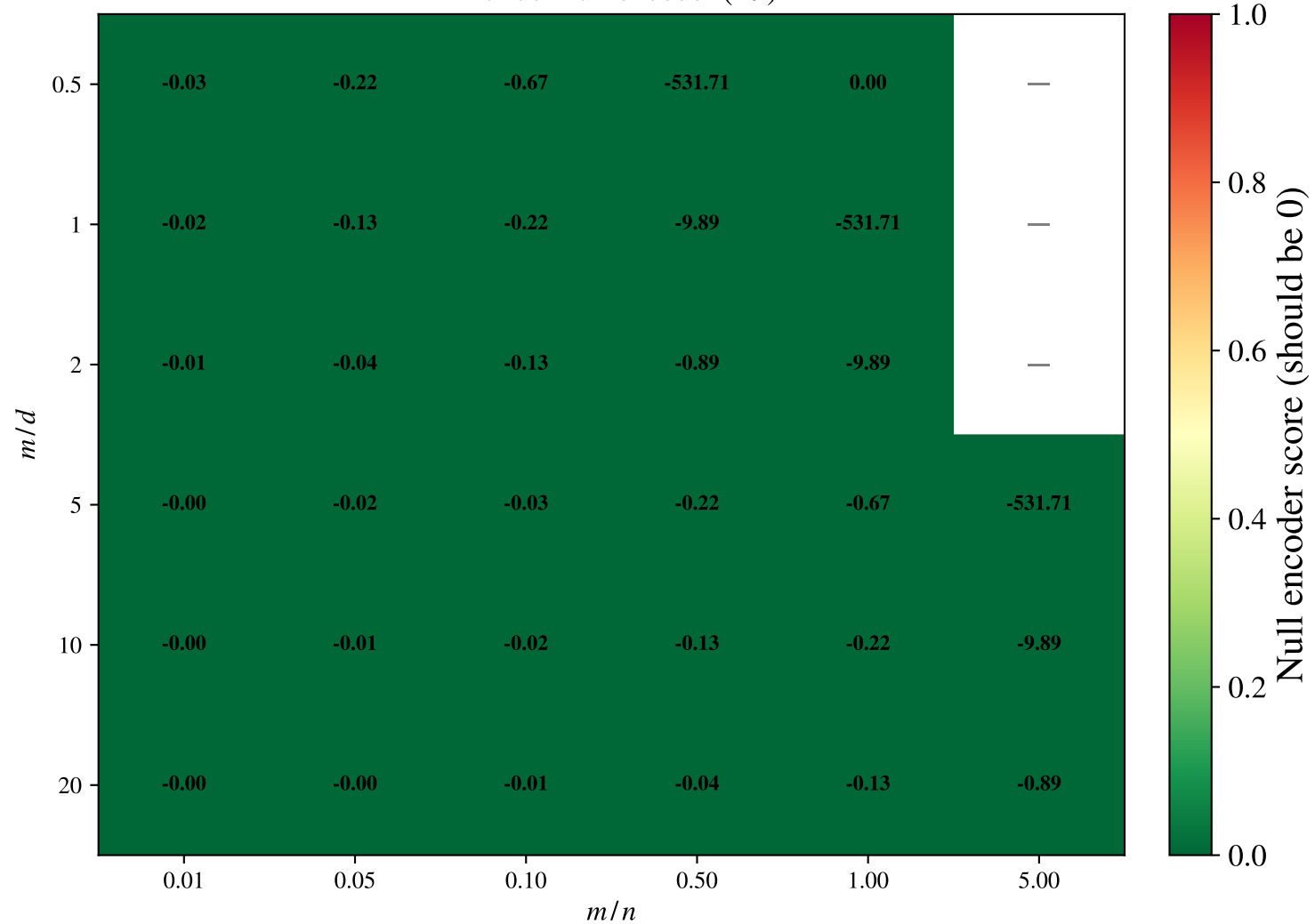
R^2 under null encoder (E9)
