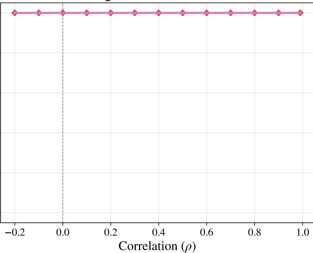
Sign-sensitive metrics
