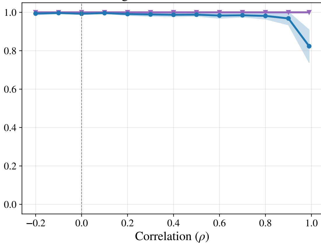
Sign-invariant metrics
