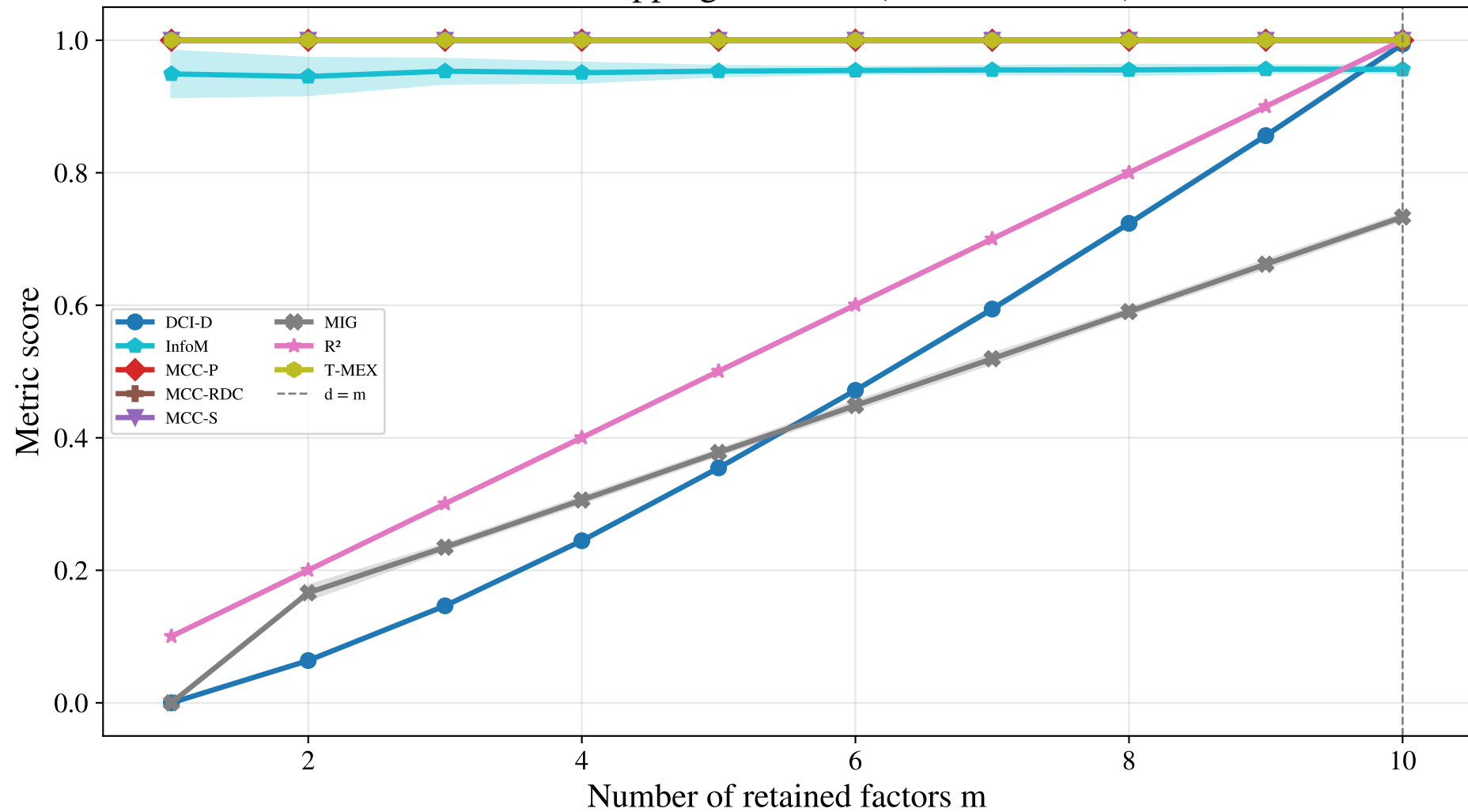
Effect of dropping variables (D1 + E4, d=10)
