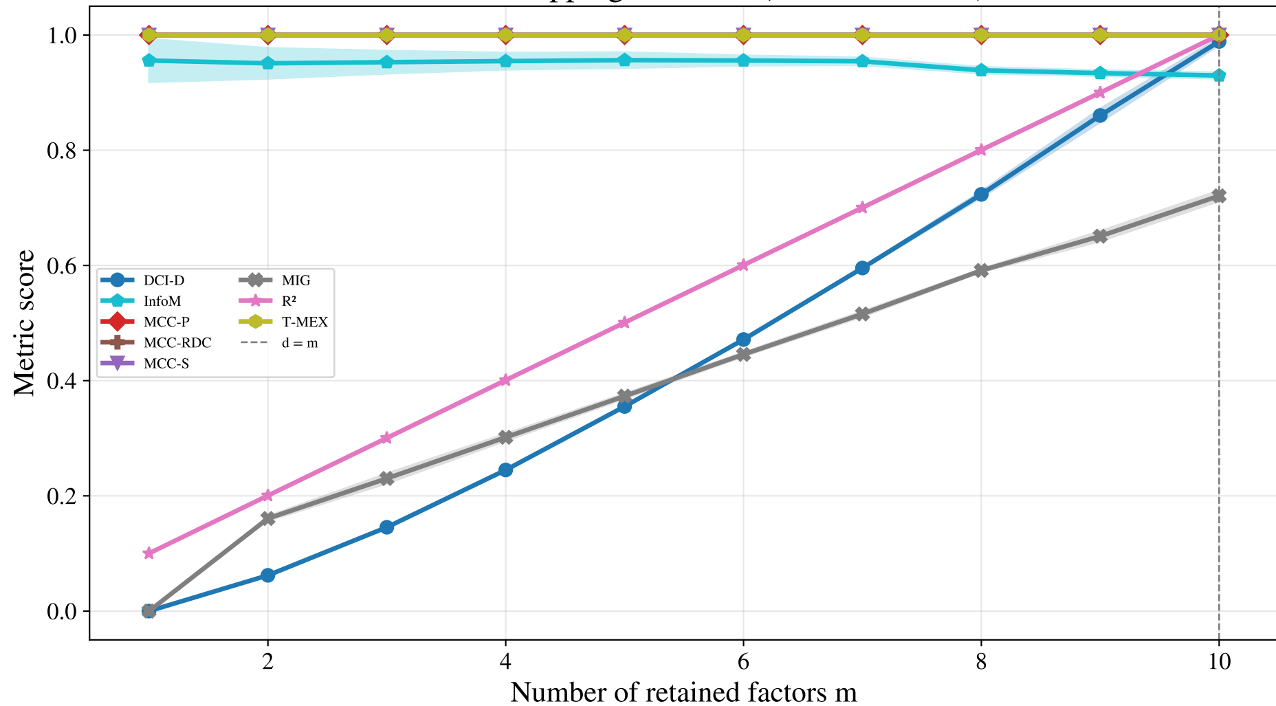
Effect of dropping variables (D4 + E4, d=10)
