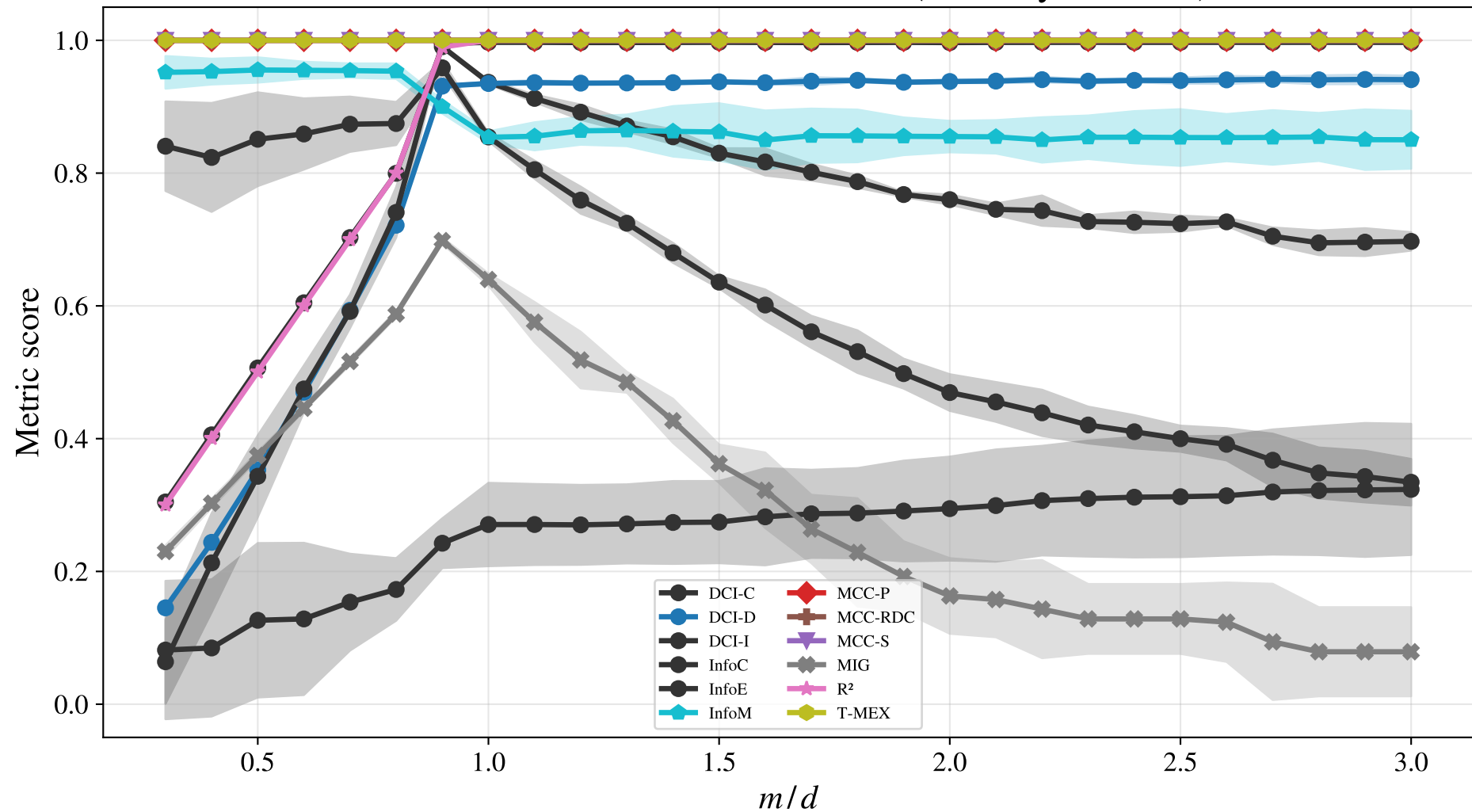
Metric score vs structural ratio m/d (D3, vary m , d=10 )
