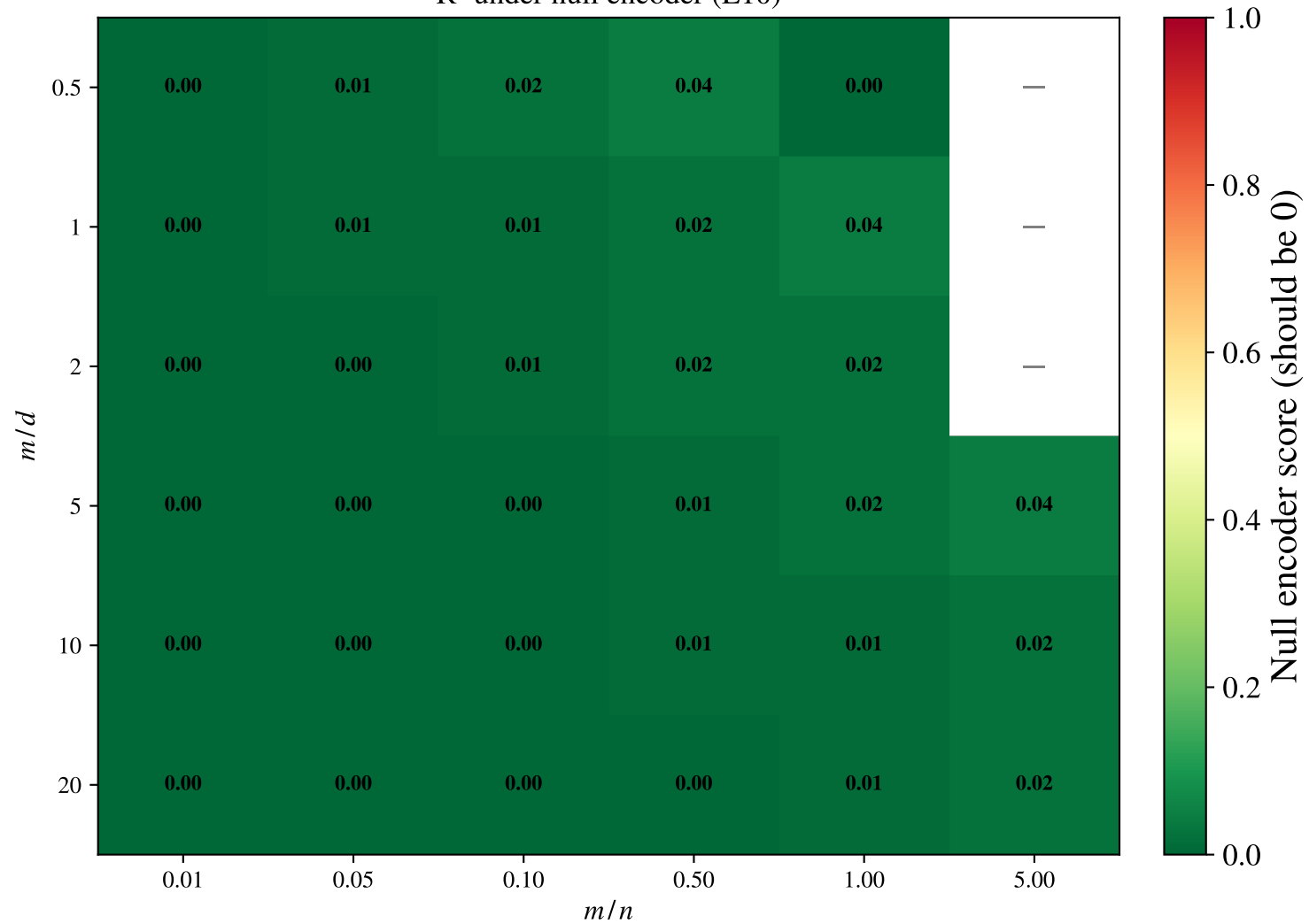
R 2 under null encoder (E10)
