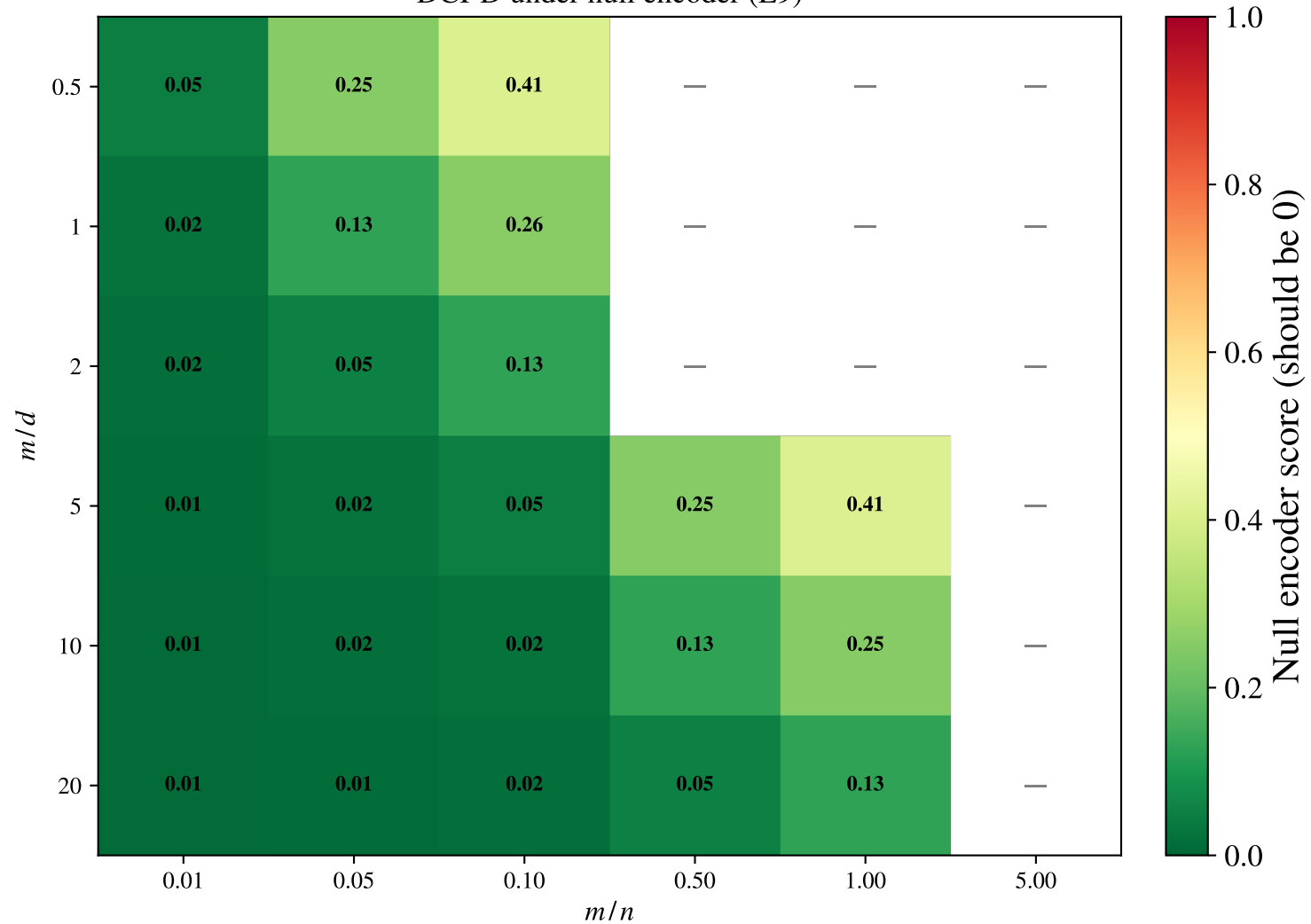
DCI-D under null encoder (E9)
