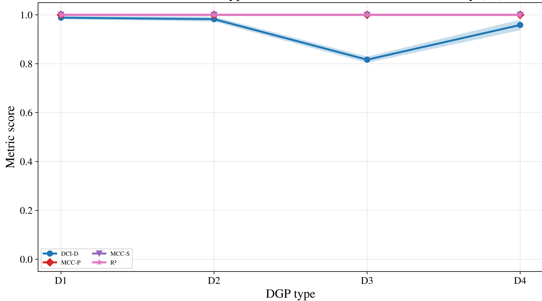
Metric invariance to DGP type under exact element-wise identifiability (E1)
