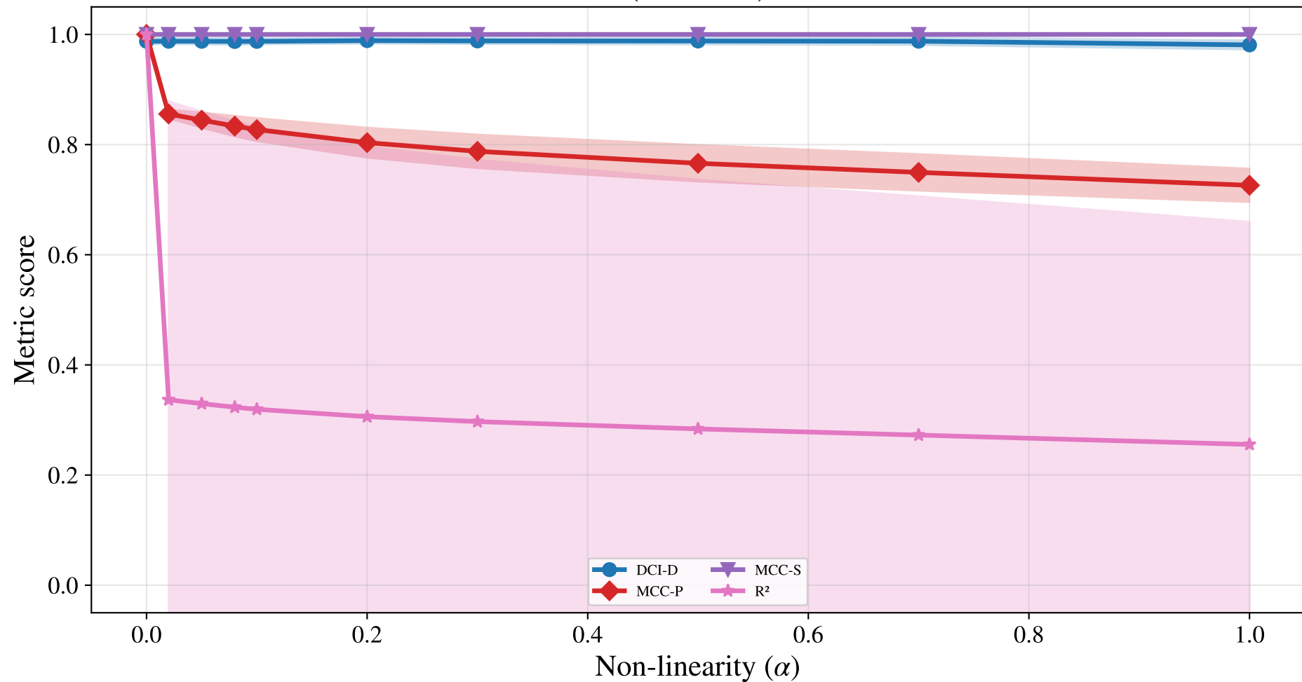
Metric sensitivity to non-linearity (averaged over function types) (D1 + E2)
