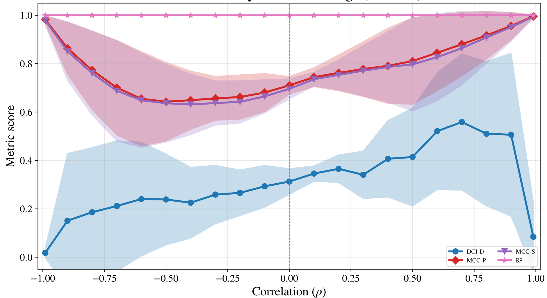
Metric sensitivity to correlation sign (D2 + E3)
