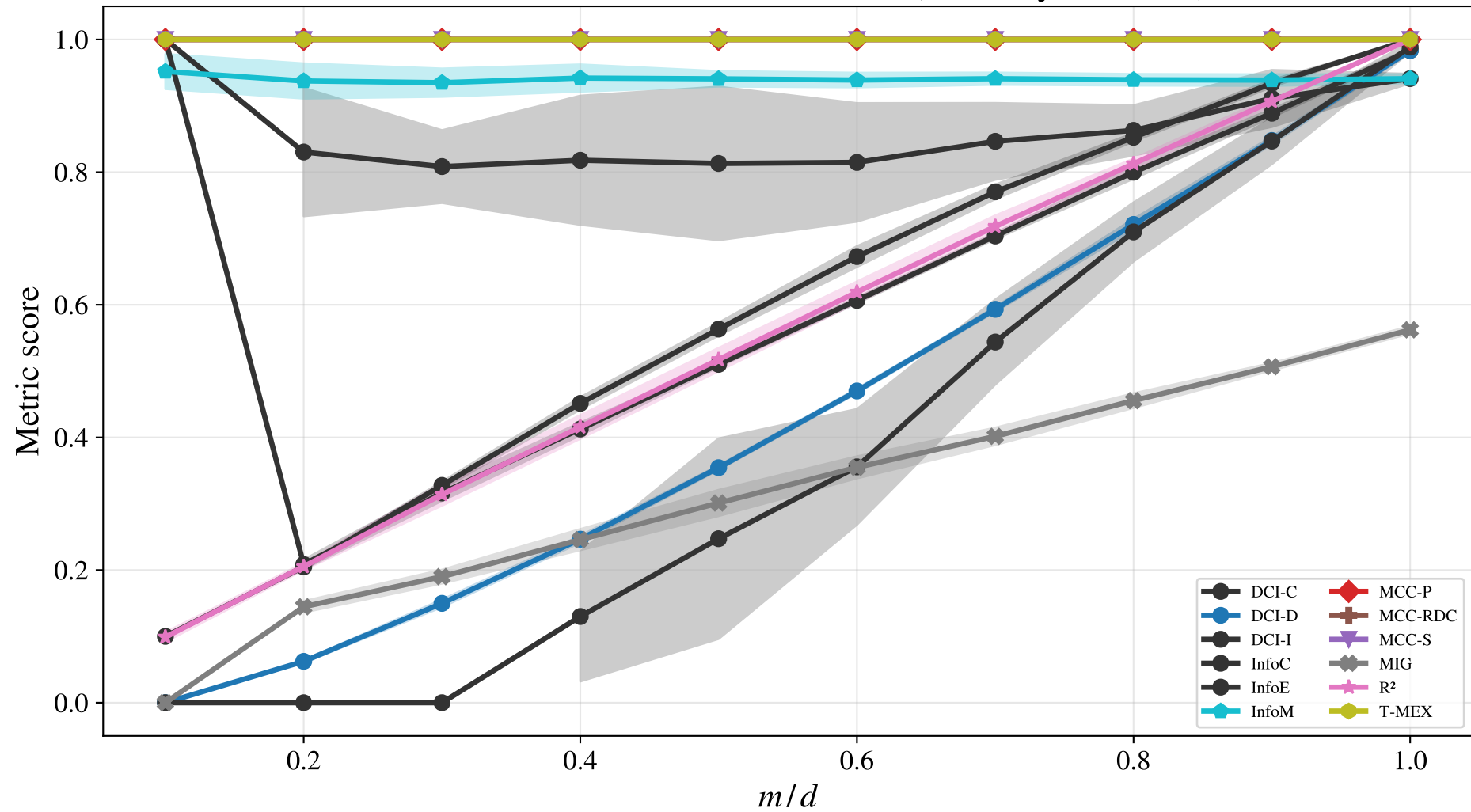
Metric score vs structural ratio m/d (D1, vary m , d=10 )
