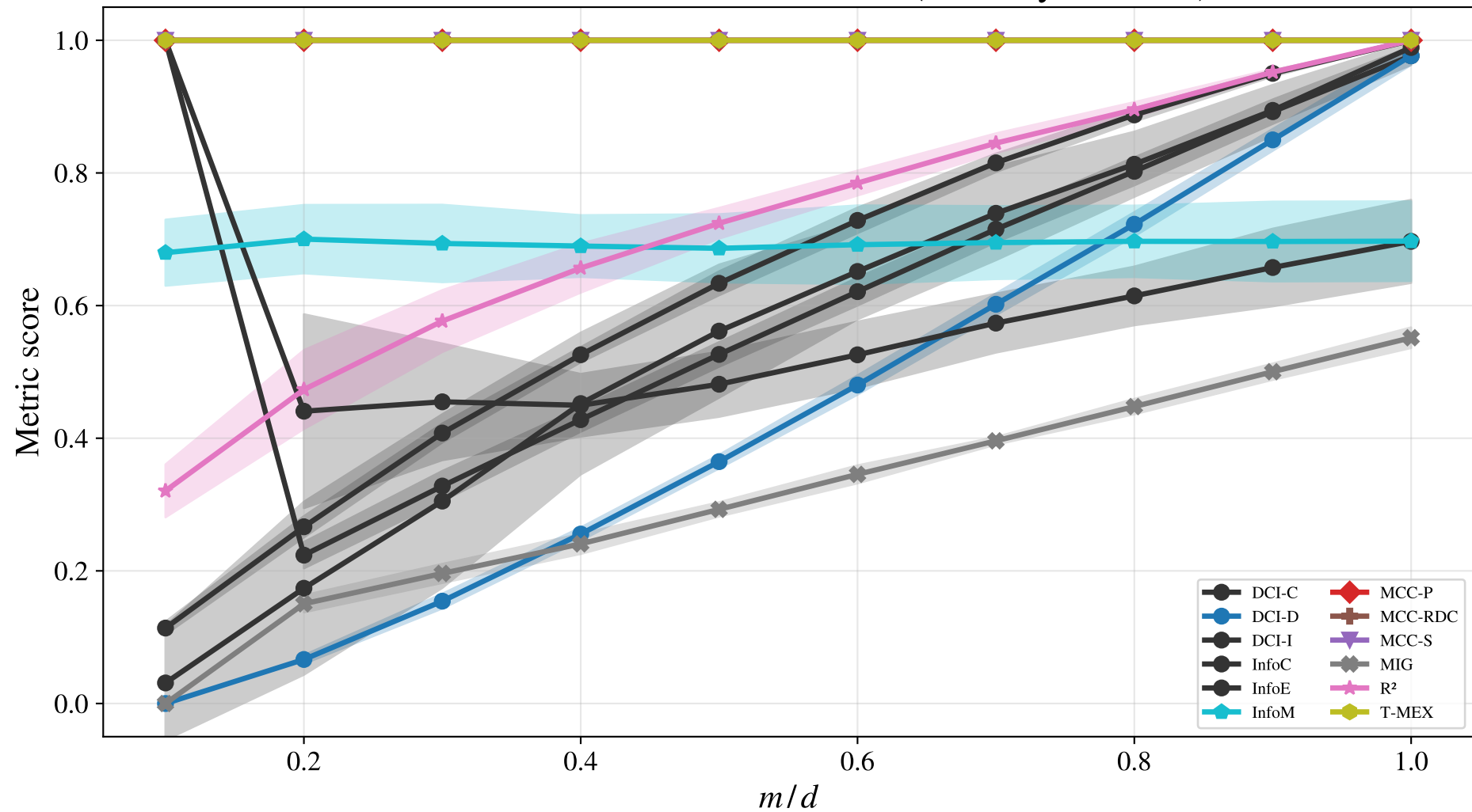
Metric score vs structural ratio m/d (D2, vary m , d=10 )
