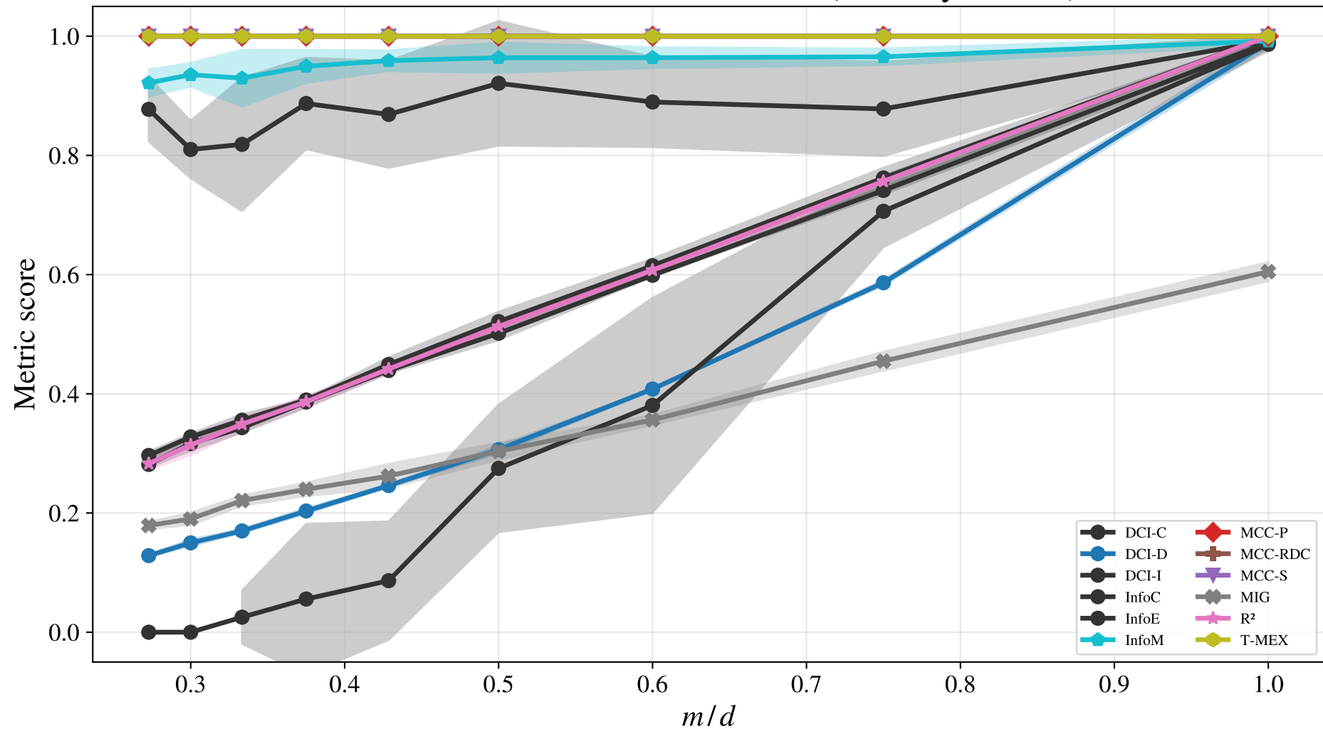
Metric score vs structural ratio m/d (D1, vary d , m=3 )
