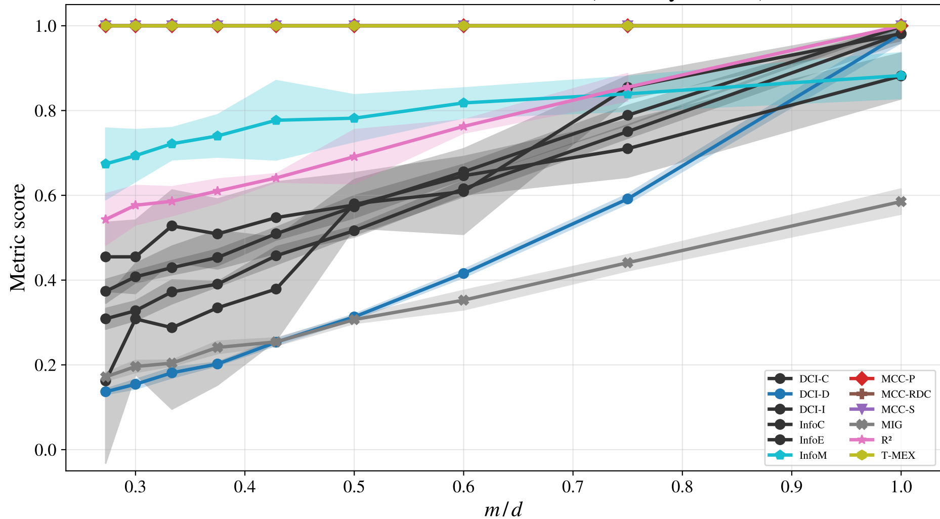
Metric score vs structural ratio m/d (D2, vary d , m=3 )
