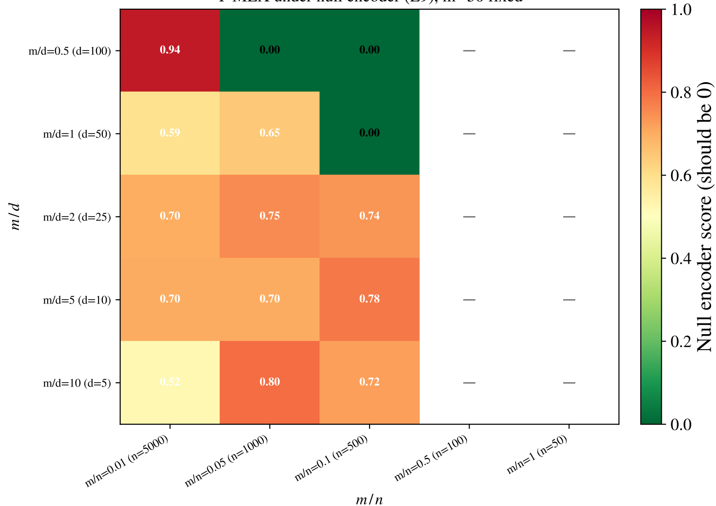
T-MEX under null encoder (E9), m=50 fixed
