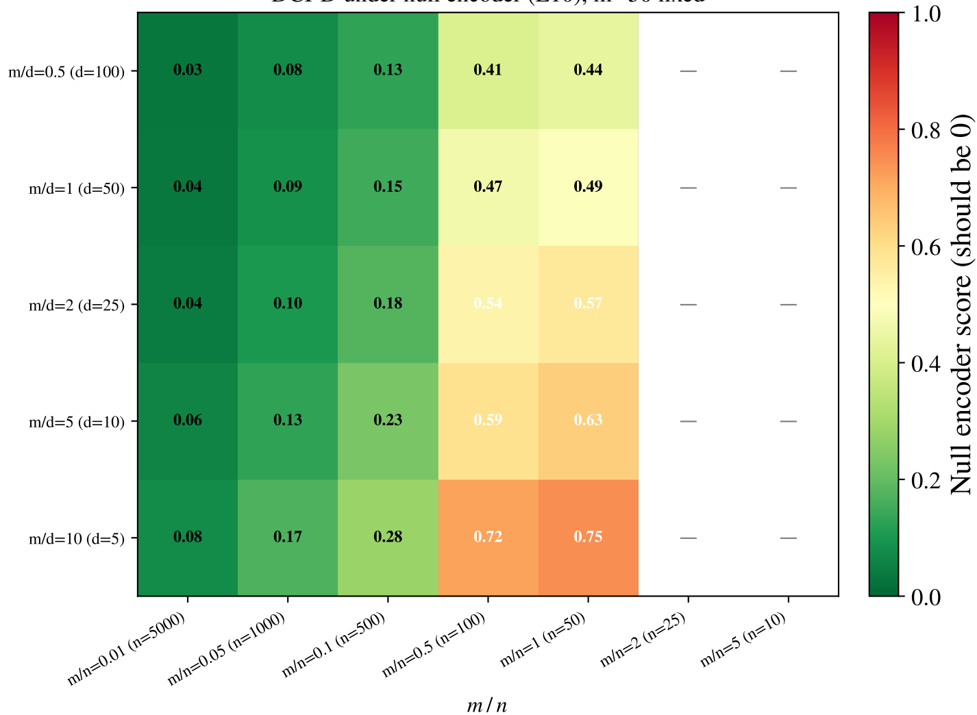
DCI-D under null encoder (E10), m=50 fixed
