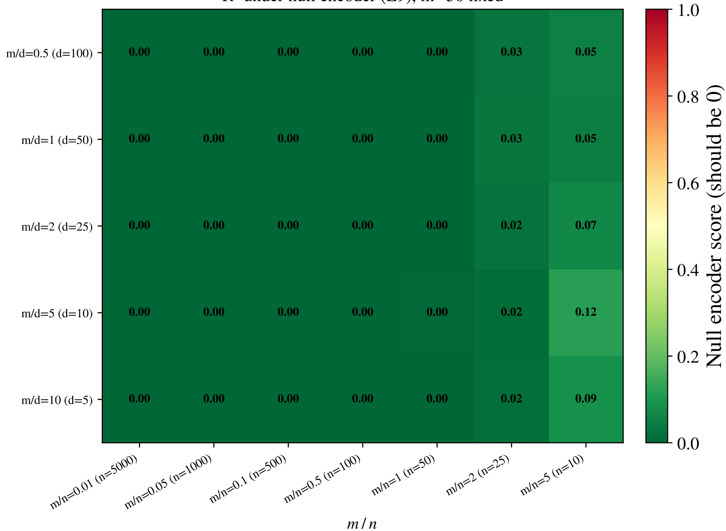
R^2 under null encoder (E9), m=50 fixed
