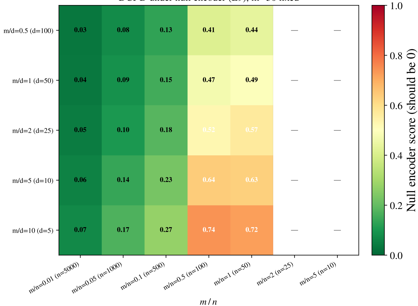
DCI-D under null encoder (E9), m=50 fixed
