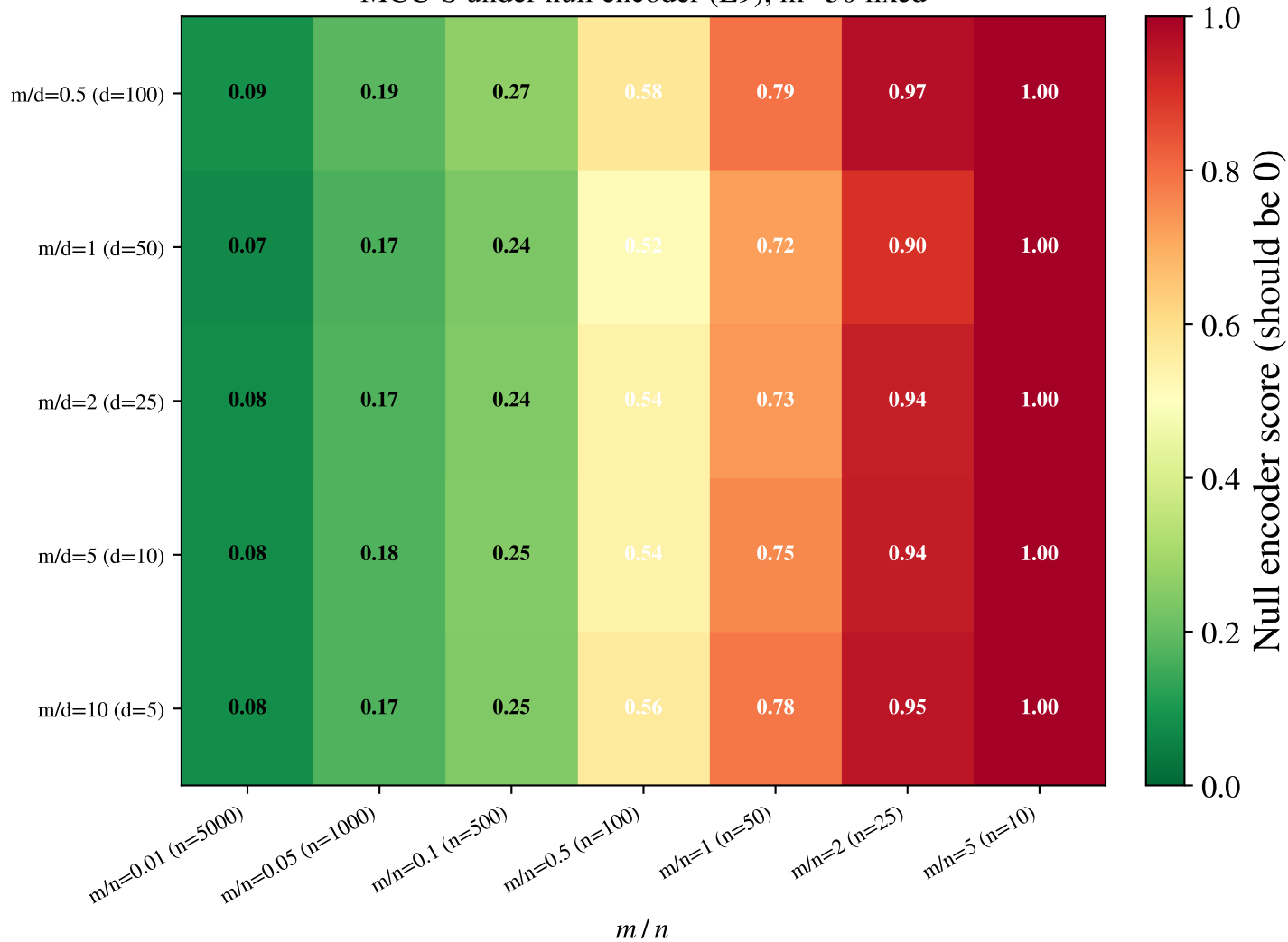
MCC-S under null encoder (E9), m=50 fixed
